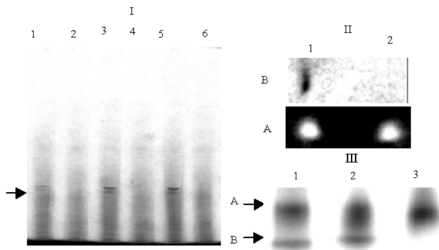
Fig. 4 I and II: In-gel activity staining of two Fe-S containing enzymes of the TCA cycle by BN-PAGE. I. In-gel activity staining of ACN in increasing protein concentrations. Lanes 1 and 2, 3 and 4 and 5 and 6 contain 60, 70 and 80 \mu\text{g} soluble CFE. Odd-numbered lanes are citrate soluble CFE while even-numbered lanes contain Al-citrate soluble CFE (reaction time: 15 min). II. 2D in-gel activity staining and 2D BN/SDS-PAGE/Western blot of ACN. Panel A: 2D BN-PAGE of ACN activity in soluble CFE. Panel B: 1D BN-PAGE, 2D SDS-PAGE (Western blot). Lane 1: soluble CFE from citrate medium; 2: soluble CFE from Al-citrate medium. III. BN-PAGE activity stain of FUM in Al-stressed CFE membranes. Lanes 1, 2 and 3: citrate media enriched with 5, 10 and 15 mM Al, respectively. (A) corresponds to FUMC while (B) corresponds to FUMA. Note the disappearance of FUMA (Fe-S protein) as the concentration of Al was increased
