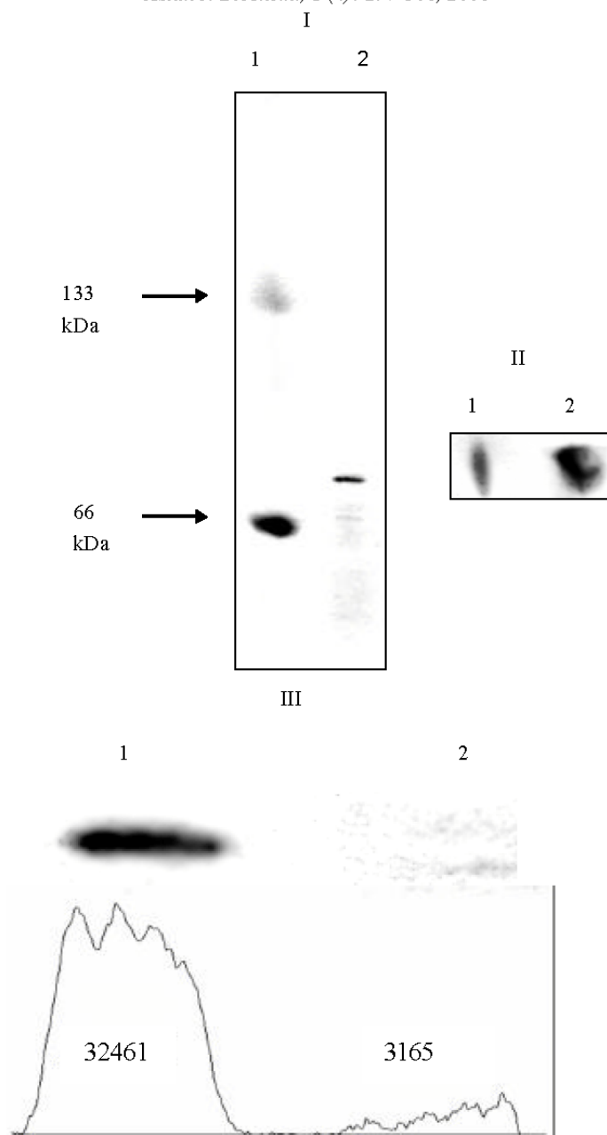
Fig. 2 I: In-gel activity staining and protein quantitation of NAD-ICDH by BN-PAGE. Lane 1: BSA standard; lane 2: in-gel activity stain of NAD-ICDH from citrate membrane CFE with BN-PAGE. II. 2D PAGE analysis of NAD-ICDH in the membrane CFE. Lane 1: 2D PAGE in-gel activity staining (1D BN-PAGE and 2D CN-PAGE). Lane 2: silver stain of 1D BN-PAGE followed by 2D SDS-PAGE. Slabs of gel from the 1D were soaked in 1% SDS and 1% 2-mercaptoethanol for 2 h before running the 2D. III. In-gel activity and quantitation of NAD-ICDH. Lane 1: citrate membrane CFE; 2: Al-citrate membrane CFE; Band intensity was quantified with Scion Image
